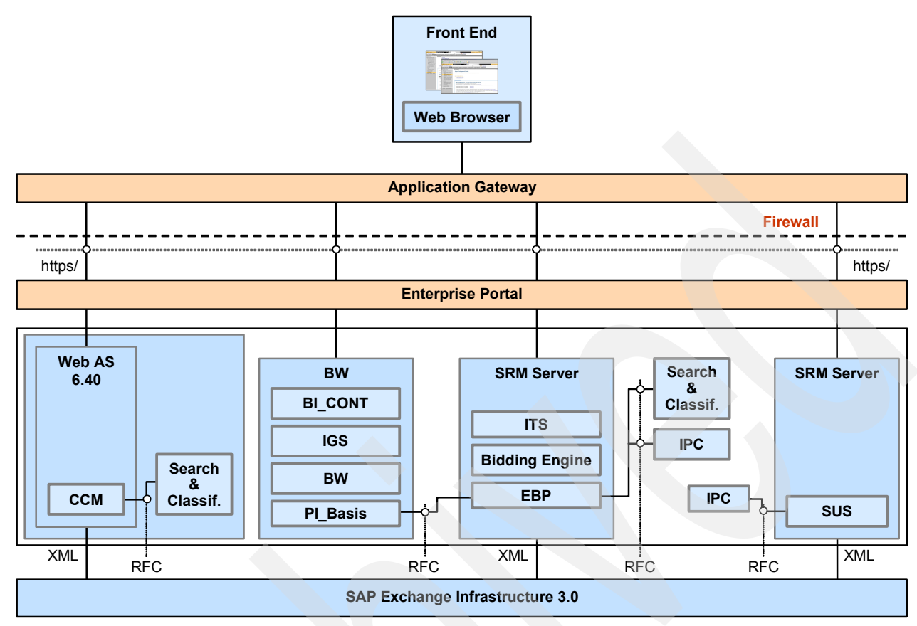
Figure 5-14 mySAP SRM Self-service procurement technical landscape
