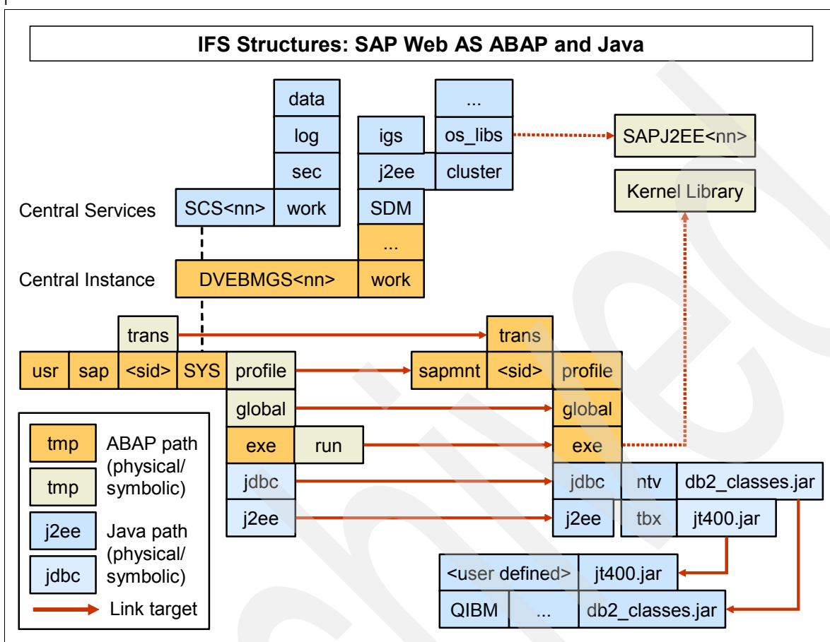
Figure 6-2 IFS structures for the Web Application Server, ABAP and Java
