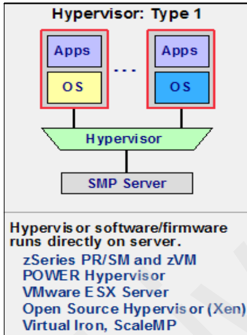
Figure 2-7 Type-1 hypervisor
