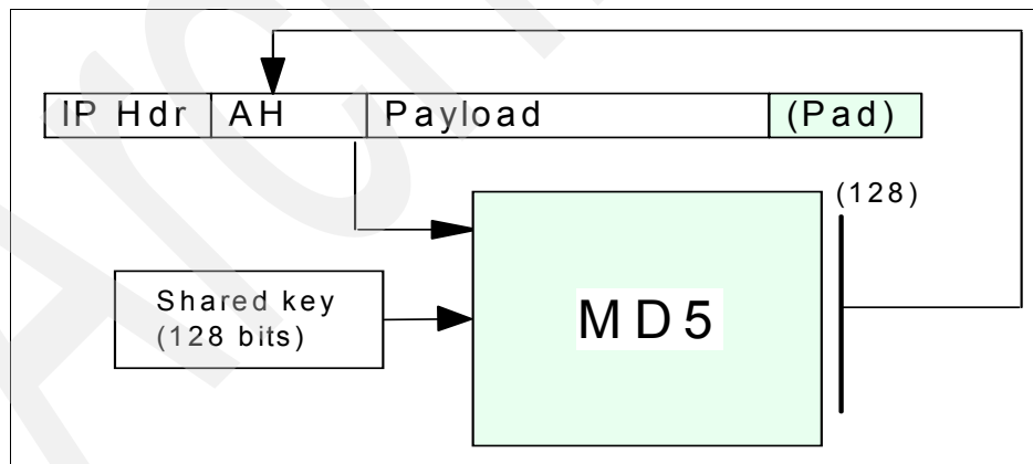
Figure 22-7 Keyed MD5 processing
