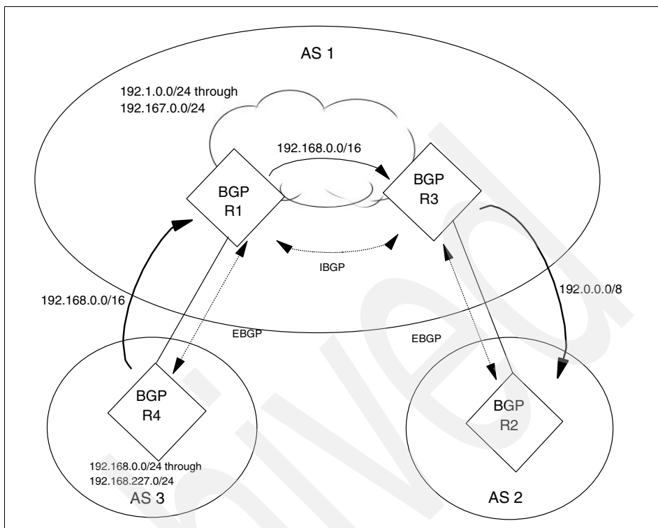
Figure 5-27 BGP route aggregation
