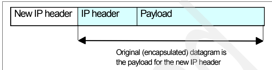
Figure 22-23 IP tunneling
