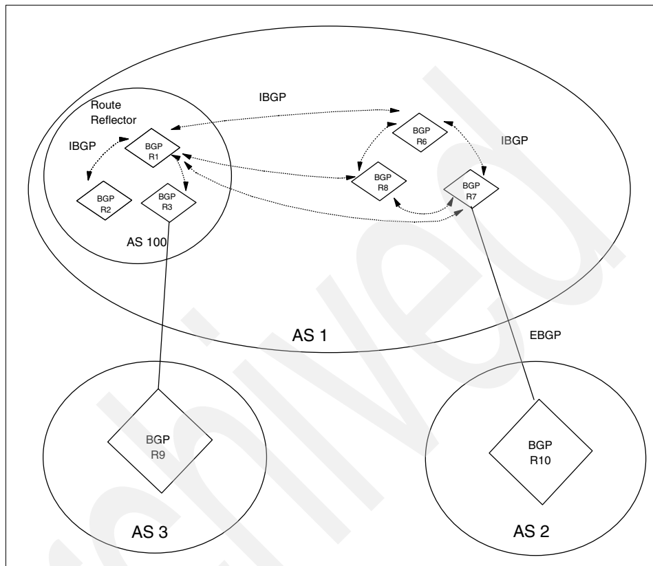
Figure 5-29 BGP route reflector
