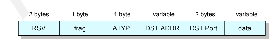
Figure 22-48 SOCKSv5: UDP datagram request header format
