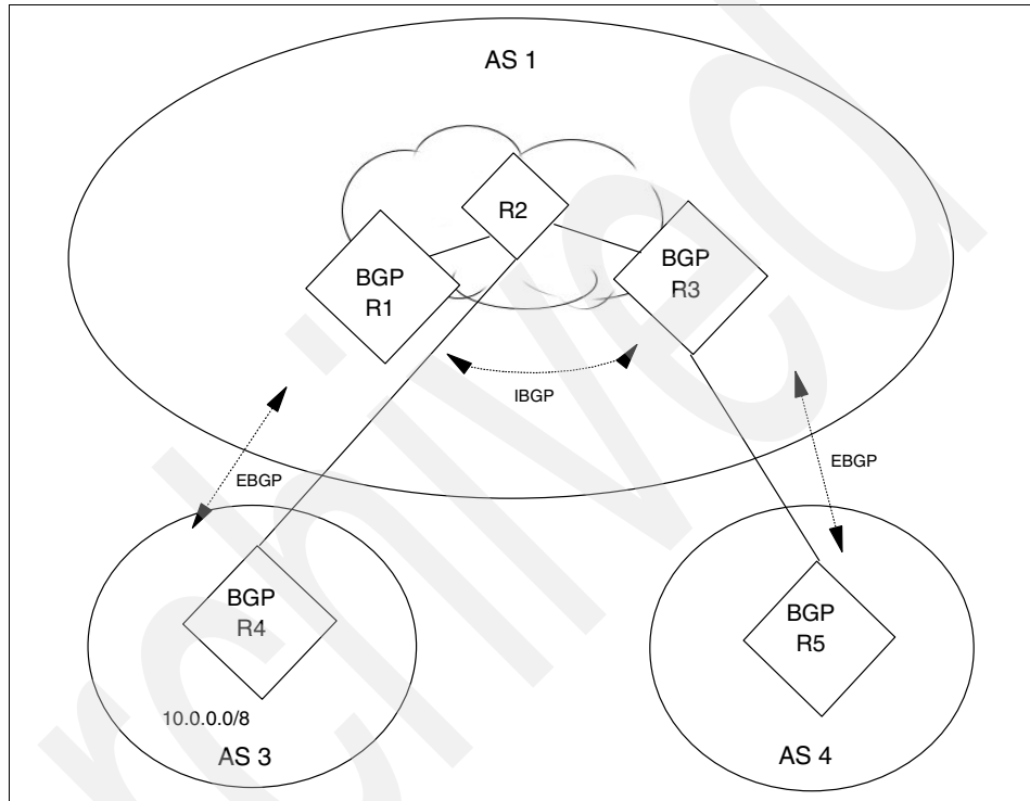
Figure 5-26 BGP synchronization
