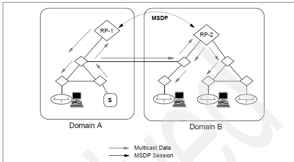
Figure 6-14 MSDP operations
