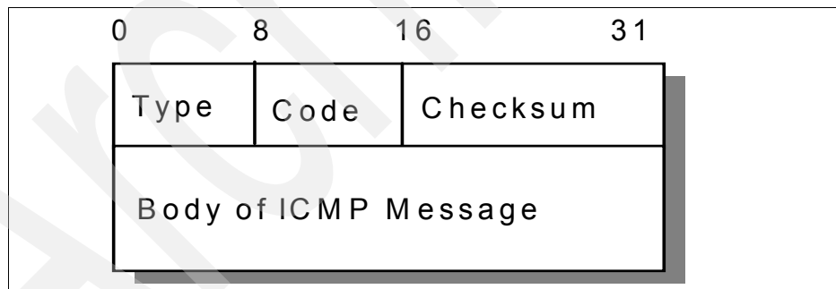
Figure 9-14 ICMPv6 general message format
