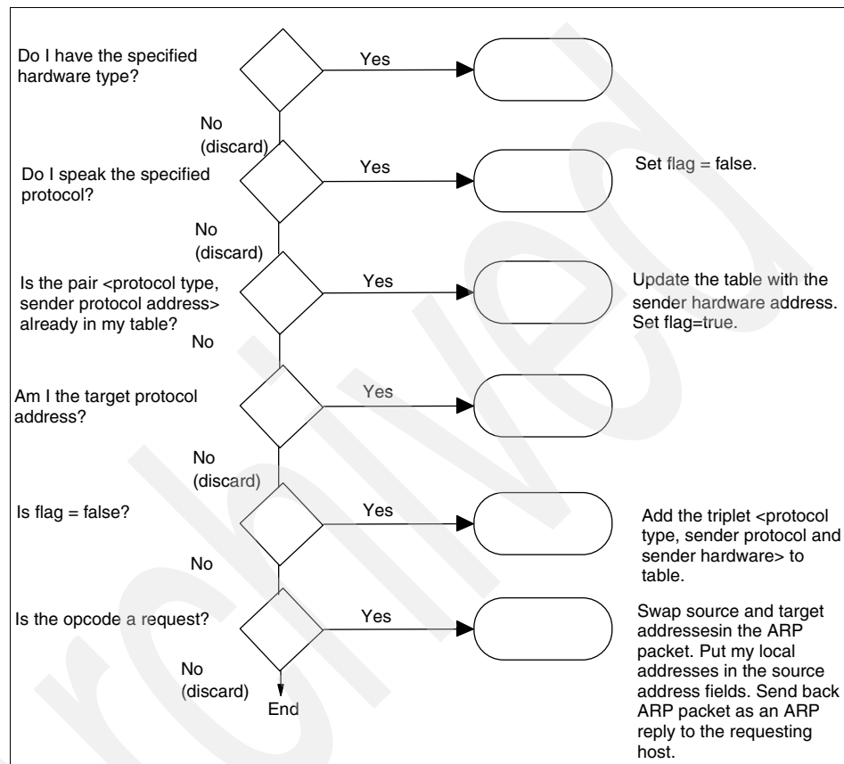
Figure 3-40 ARP: Packet reception
