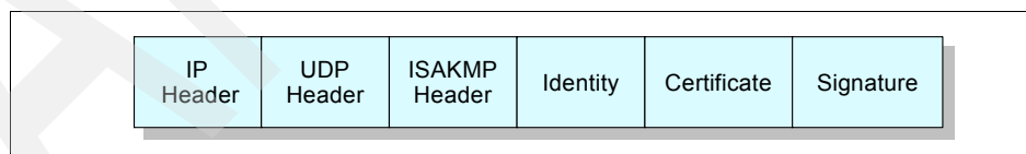
Figure 22-40 Message 5 of an ISAKMP phase 1 exchange
